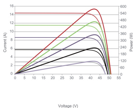
Current-Voltage & Power-Voltage Curves (575W)
